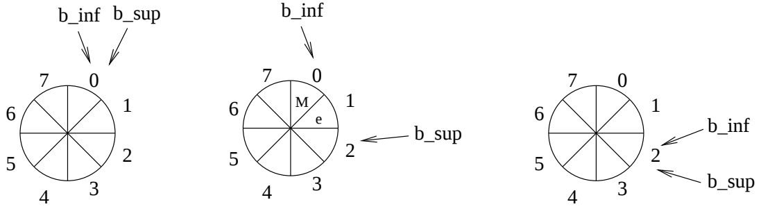
Figure 8: Operation on buffer
