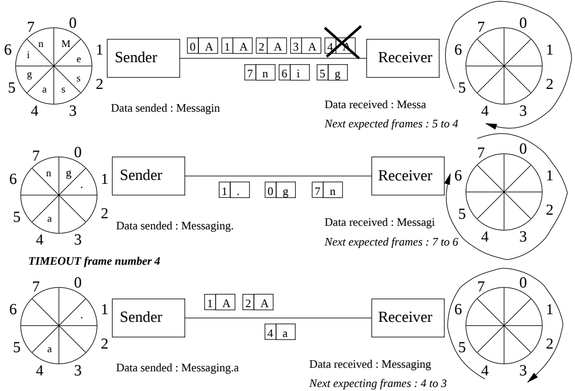
Figure 10: Limite du Protocole Anticipation Window
