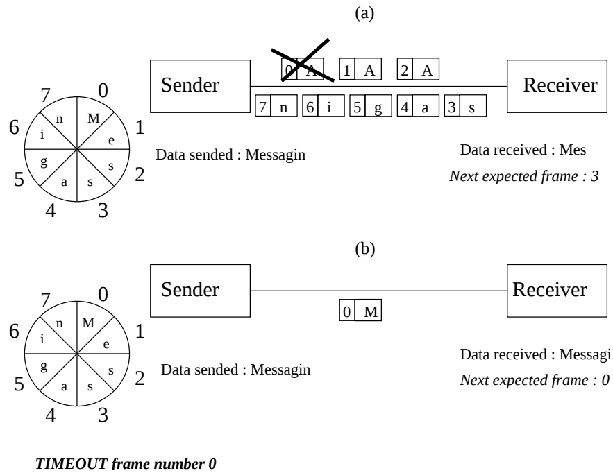
Figure 7: Sliding Window protocol limitation
