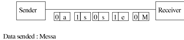
Figure 2: Bit Alternate Protocol
